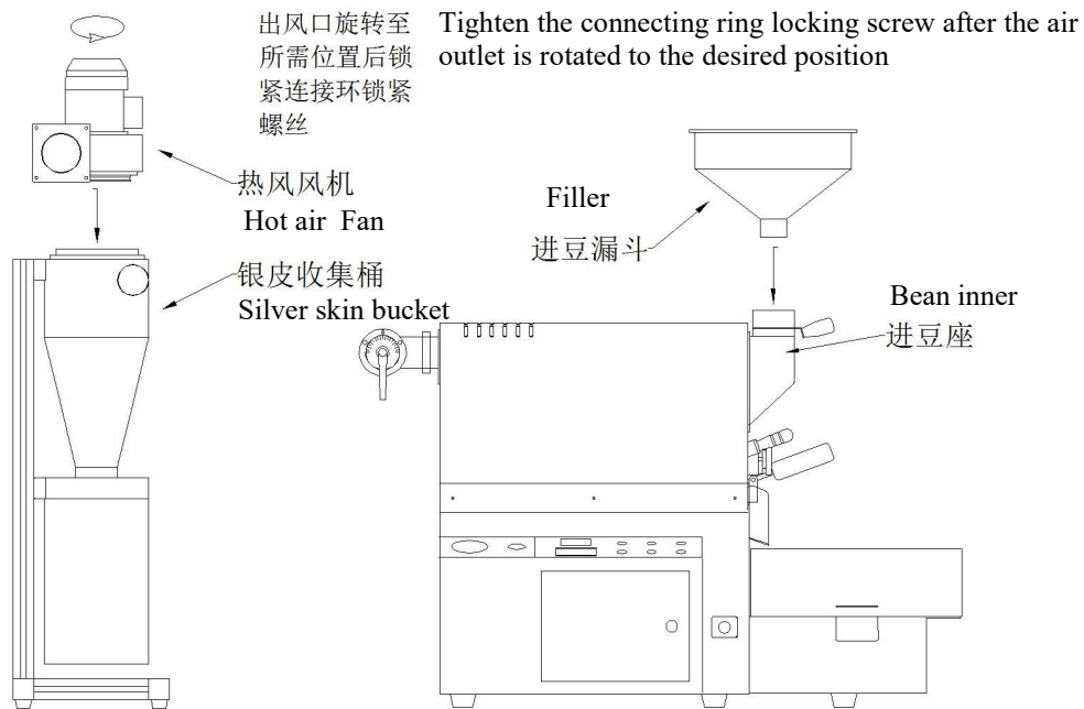
Diagram of roaster installation connection
